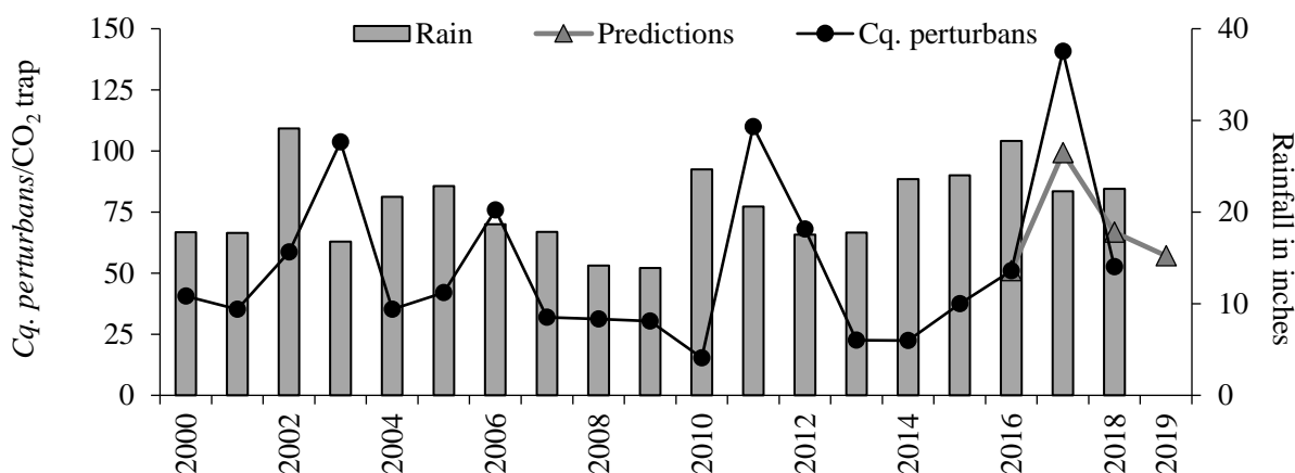
Figure 1.13 Average number of Coquillettidia perturbans in CO 2 traps and average seasonal rainfall per gauge, 2000-2018. The gray line shows the predicted amounts for 2017, 2018, and 2019.
