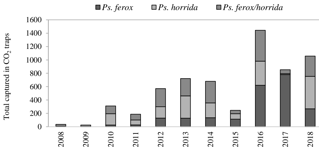
Figure 1.17 Total yearly Ps. ferox , Ps. horrida and Ps. ferox/horrida collected from Monday Night CO 2 traps (low, high and any outside District), 2008-2018.
