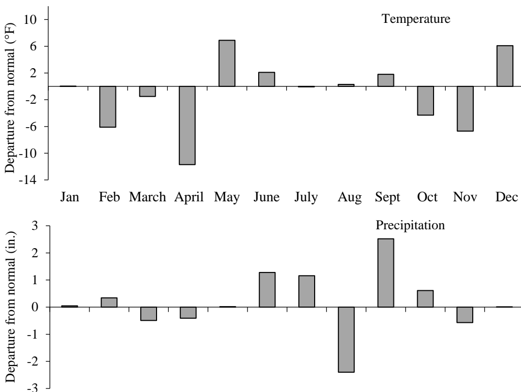
Figure 1.2 Monthly departures from normal for temperature and precipitation January-December, 2018 (source: National Weather Service, Twin Cities Station).
