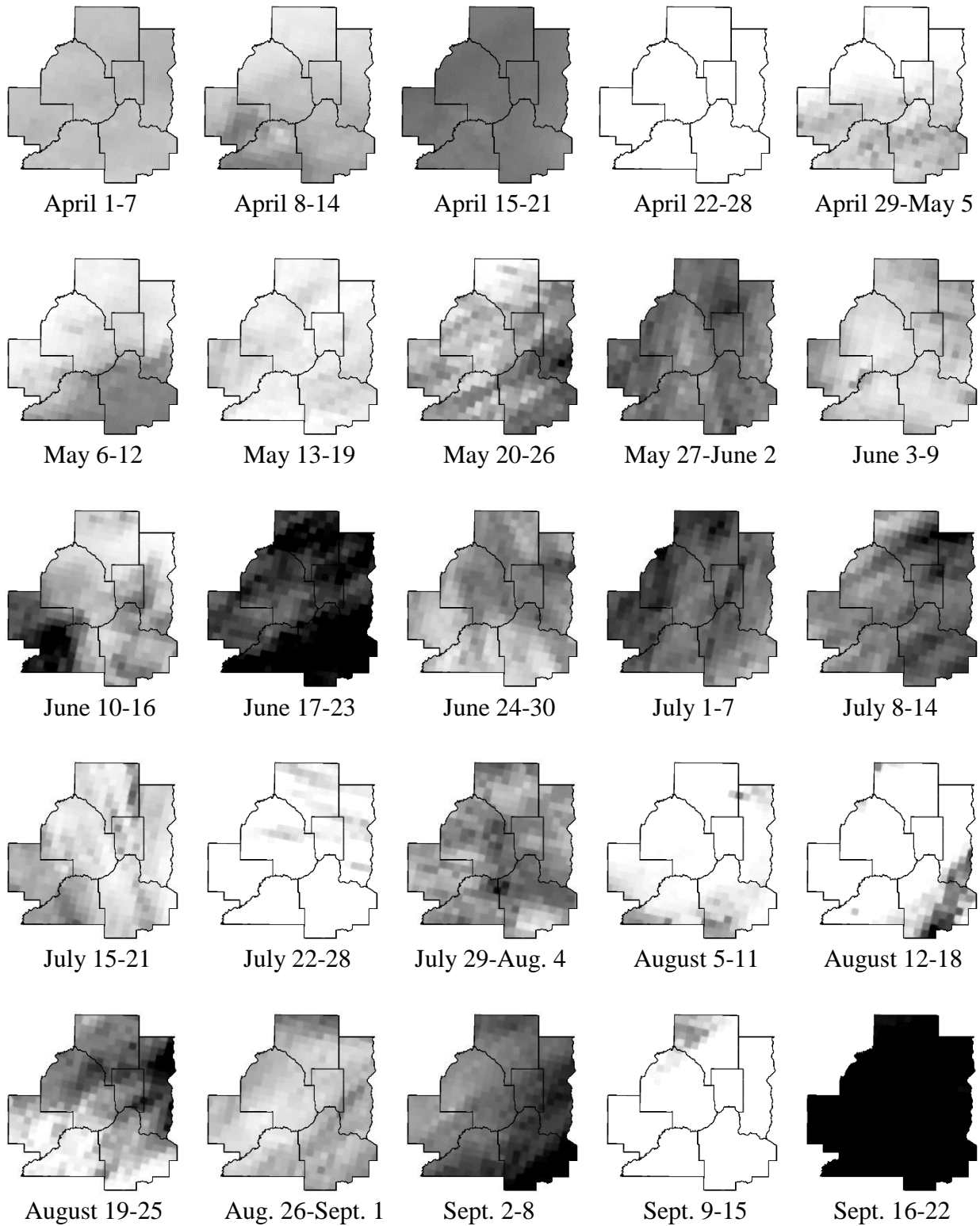
Figure 1.3 Weekly rainfall in inches, 2018. RFC-corrected data using 406 4x4 km grid cells. Inverse distance weighting was the interpolation method used for shading the maps.
