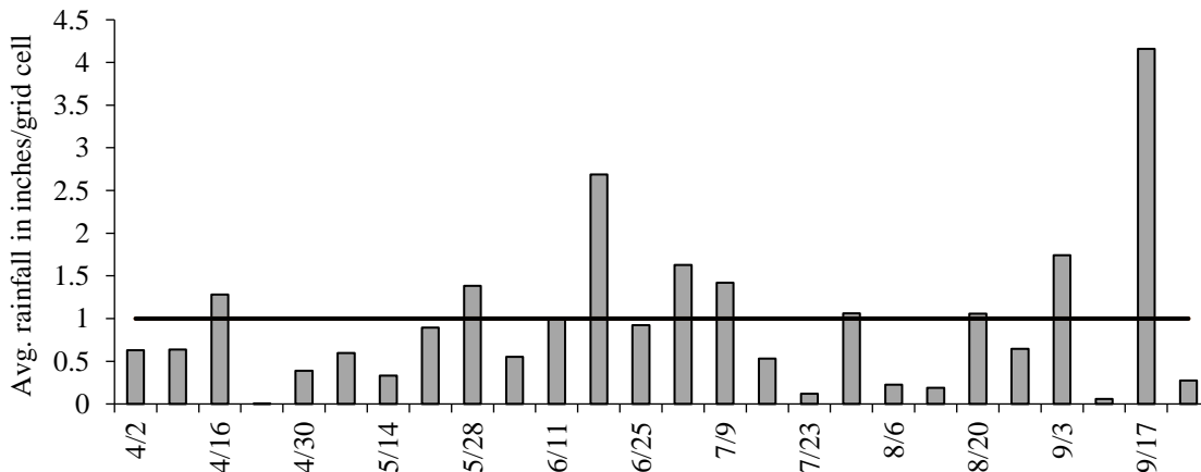
Figure 1.1 Weekly rainfall amounts per grid cell, 2018 (RFC data). Dates represent the Monday of each week. Solid line indicates 1-inch, the amount sufficient to induce egg-hatch.
