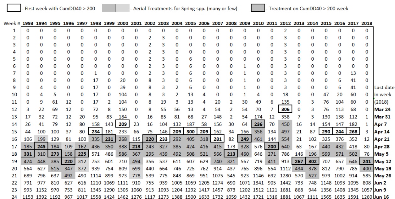
Figure 7.4 Cumulative Degree Days (base 40 °F, 4.4 °C) from January 1, MSP Airport.
